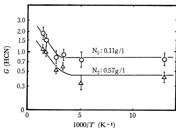
Fig. 3. Arrhenius' plot of G(\text{HCN}) . \gamma -rays; 6.8 \times 10^6 R/hr, 0–6 hr irradiated, \text{C}_2\text{H}_4/\text{N}_2 = 0.075 . \bigcirc ; \text{N}_2 gas density = 0.11 g/l. \triangle ; \text{N}_2 gas density = 0.57 g/l.
